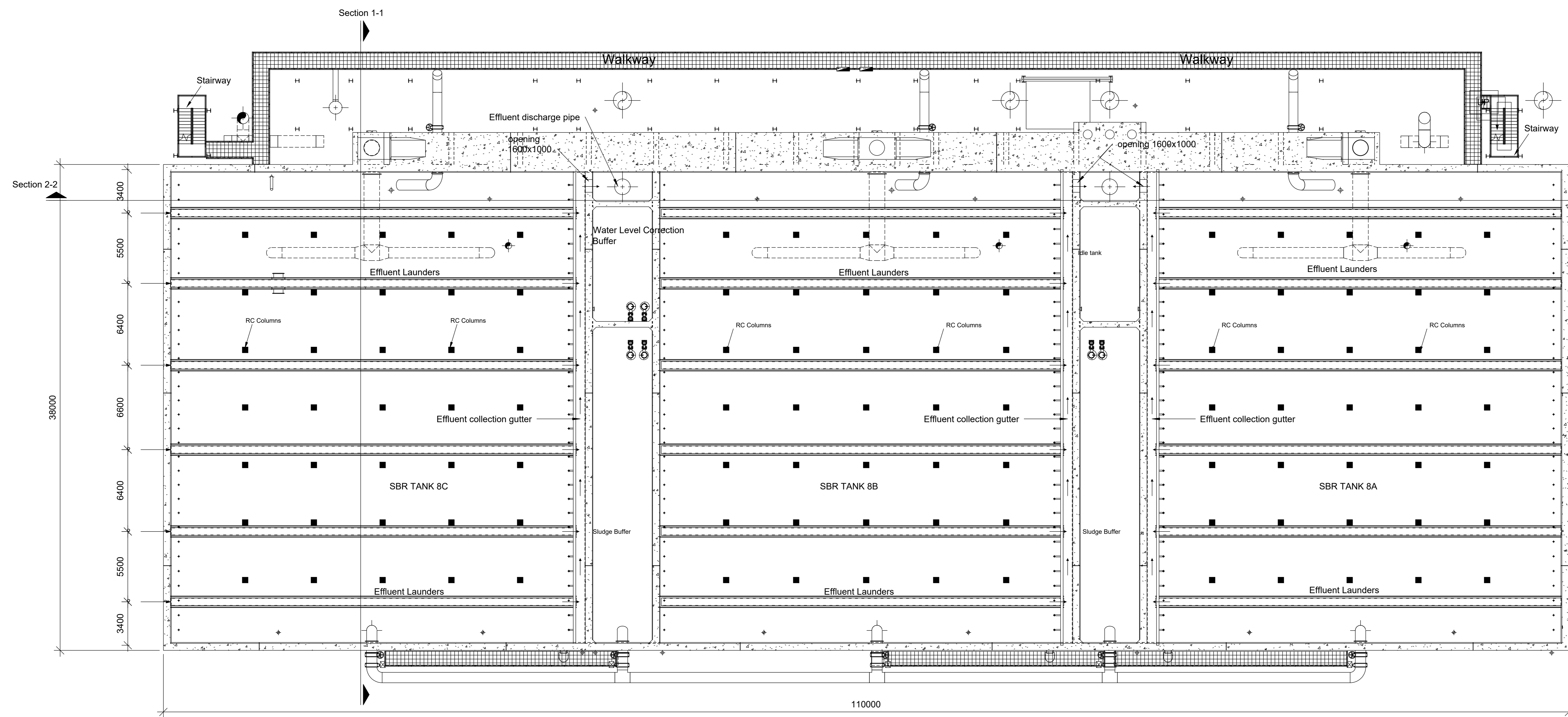
G.A. PLAN OF CAPACITY EXPANSION @ 12.400m AMD Scale 1:150
