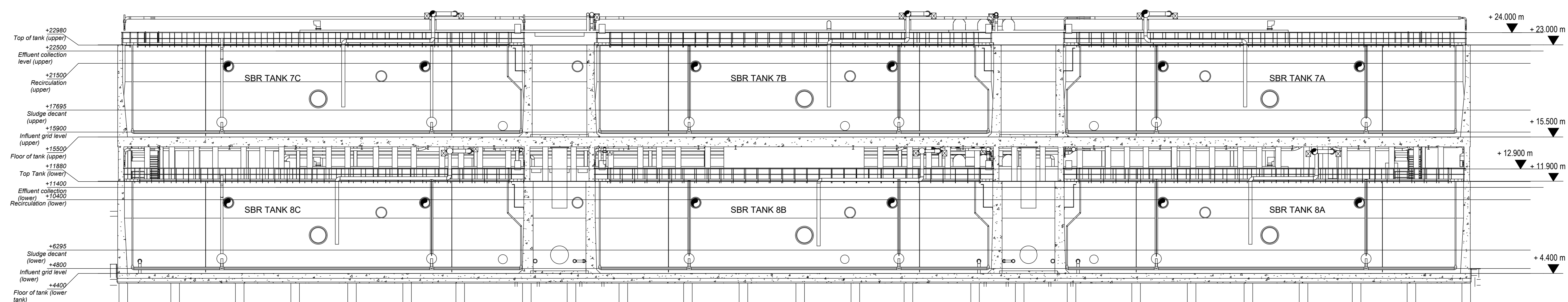
SECTION 2-2 Scale 1:150
